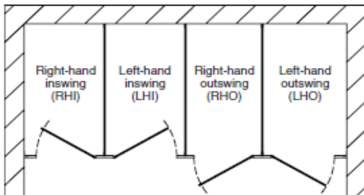
Door Hardware
