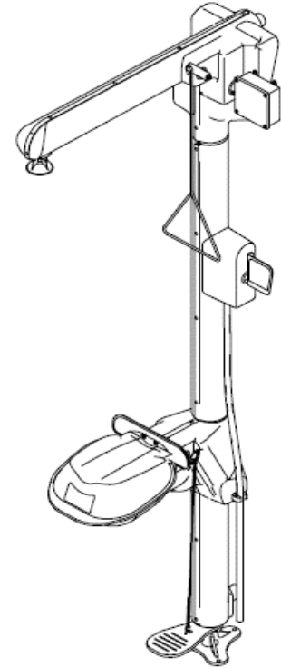
General Area unit shown with Drench Hose and Foot Pedal Activation
